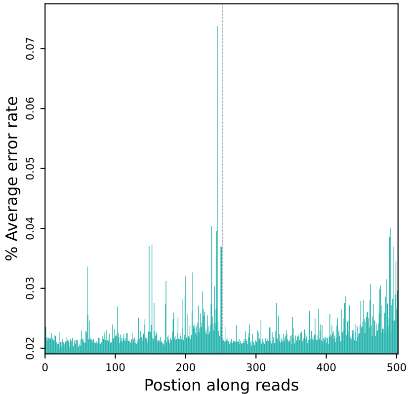
Error rate distribution along reads (R10901)
